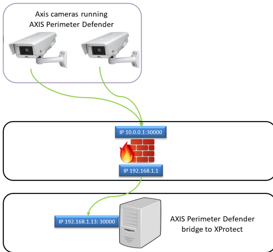
A typical NAT situation
